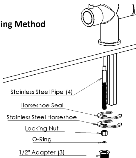
Tap Connections
